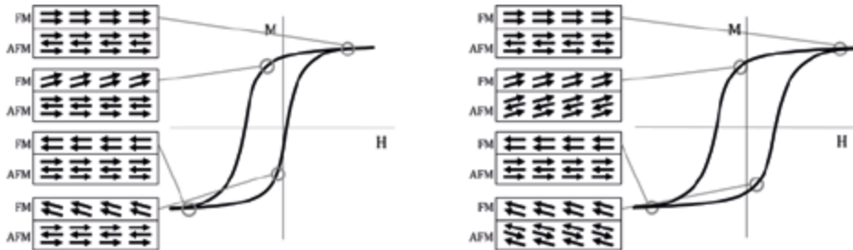
Figure 2.15: Schematic diagram of magnetic behaviour during a hysteresis loops for a AFM-FM spins system with large K_{AFM} (left) and with small K_{AFM} (right). (Nogués et al. 2005)
