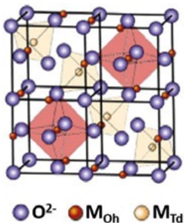
Figure 4.1: Schematic representation of the spinel crystallographic structure composed on fcc O^{2-} framework where metal ions occupy octahedral ( M_{Oh} ) an tetrahedral cavities ( M_{Td} ).
