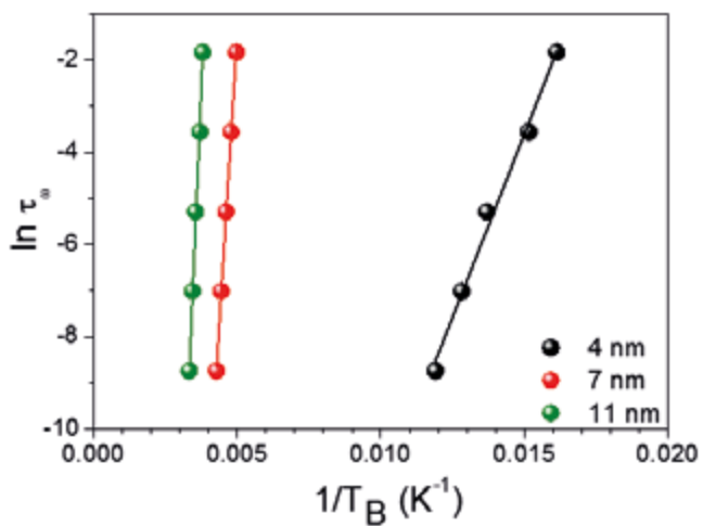
Figure 4.13: \ln \tau_\omega vs. 1/T_{B\omega} curves for 4, 7 and 11 nm cobalt ferrite nanoparticles. The straight lines represent the best fit to the Arrhenius law (Equation 4.6)
