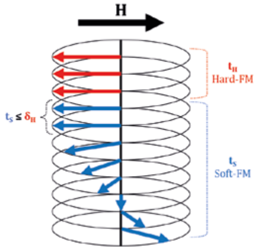
Figure 2.12: Schematic diagram of soft magnetic phase switching in a unidimensional exchange-spring magnet.
