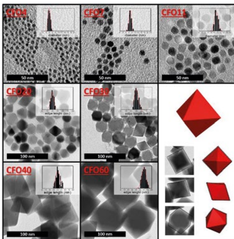
Figure 4.2: TEM images and particle size histograms for 4(1), 7(1), 11(1), 20(2), 30(4), 40(7) and 60(4) nm cobalt ferrite nanoparticle of. In the box, 2D TEM cubic, rhombohedral and hexagonal projections for octahedral nanoparticles.
