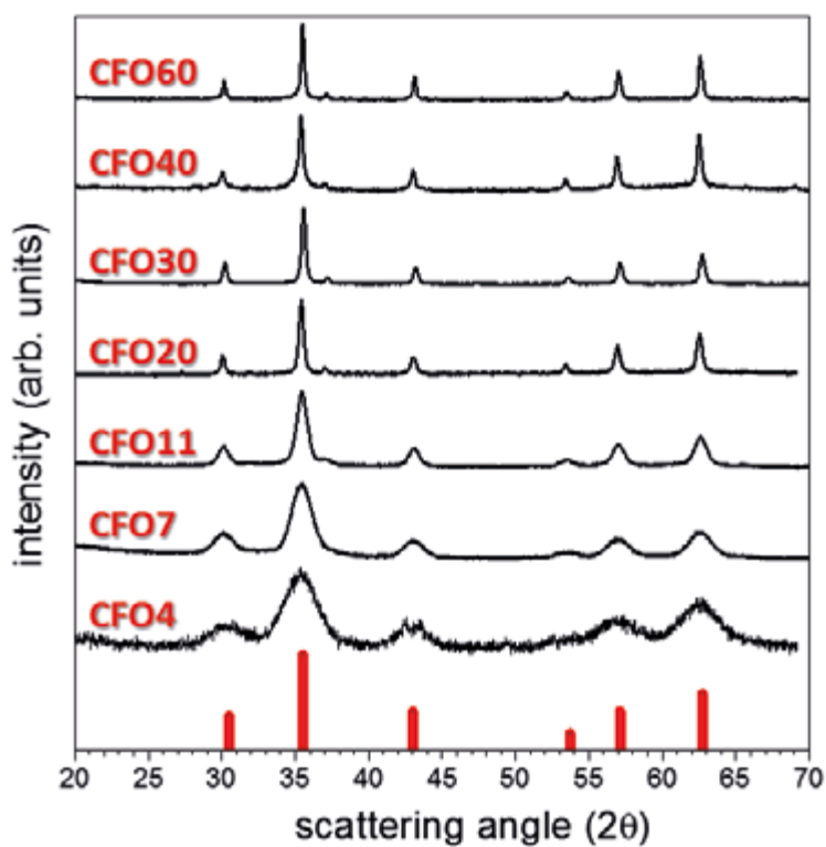
Figure 4.4: XRD patterns of the family of cobalt ferrite nanoparticles. In red is reported the reference pattern corresponding to the spinel fcc structure for \text{CoFe}_2\text{O}_4 JCPDS PDF #221086.
