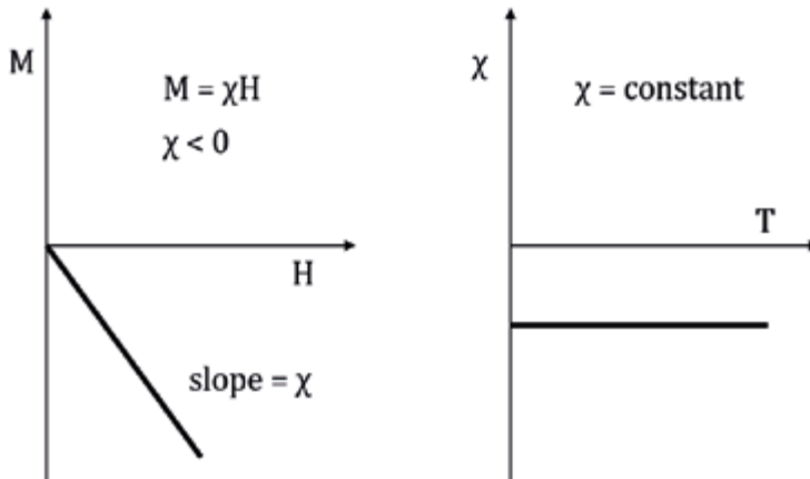
Figure 2.2: Field dependence of magnetization of diamagnetic materials (left) and temperature dependence of the magnetic susceptibility (right).
