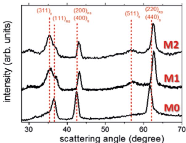
Figure 6.14: Powder XRD patterns for M0, M1 and M2 samples (indexed planes are labelled with RS and S for rock-salt and spinel structure, respectively).
