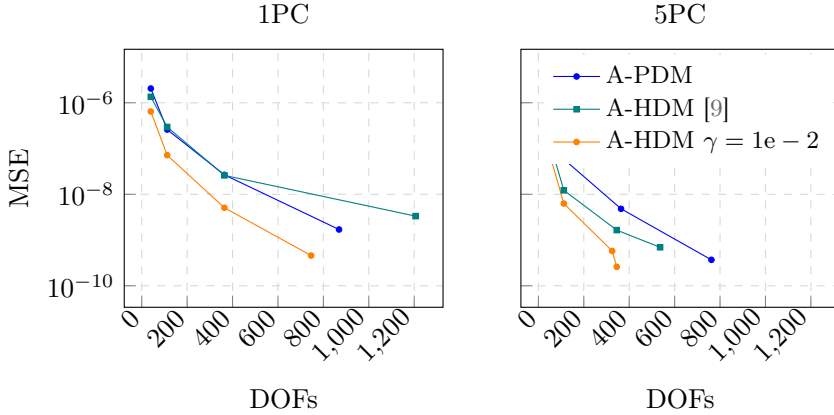
Figura 70. Adaptive spline approximation for the ship hull point cloud consisting of 3025 gridded data points parametrized with CEN method. Comparison of MSE between adaptive A-PDM (blue), A-HDM with the weights as in [9] (teal) and A-HDM with constant choice of the weights, for \gamma = 1e - 2 (orange), for 1PC (left) and 5PC (right) steps within the adaptive loop.
