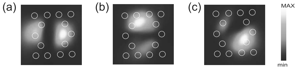
Figure 2.15: (a), (b) and (c) Spatial map of the intensity associated to the mode M2 for the polarization configuration 1, 2 and for an intermediated case, respectively. (images size 1.55 \times 1.55 \mu\text{m} ).
