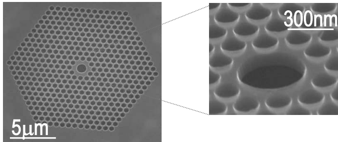
Figure 3.7: Scanning Electron Microscope image of the photonic crystal micro-cavity is provided.
