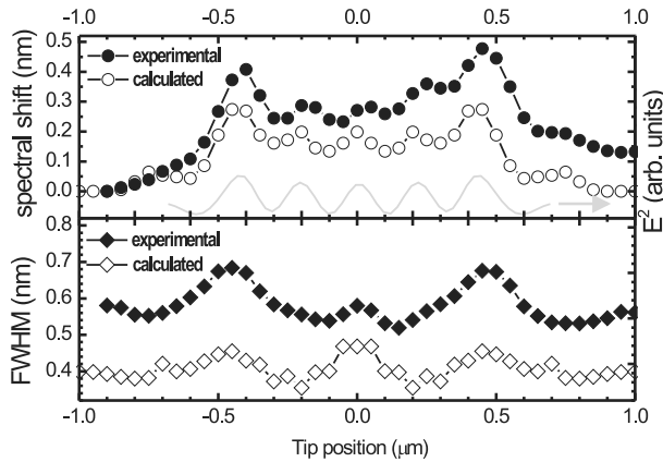
Figure 2.7: Upper panel: Experimental (filled circles) and calculated (open circles) tip-induced spectral shift of the M1 resonance. The grey line reports the vertical cross section, 200 nm wide, in the middle of the calculated electric field intensity reported in figure 2.7(b). Lower panel: Experimental (filled diamond) and calculated (open diamond) tip-induced spectral broadening of the M1 resonance.
