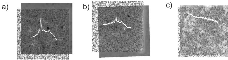
Figure 5.4: Intensity distribution of modes for samples with filling fraction of f = 30\% (a), f = 25\% (b) and f = 20\% . The white line superimposed on the image is the wavelength spectrum taken at the maximum intensity of the mode. The random dielectric matrix is superimposed to the intensity profiles together with the wavelength spectrum (white curves) of a typical mode.
