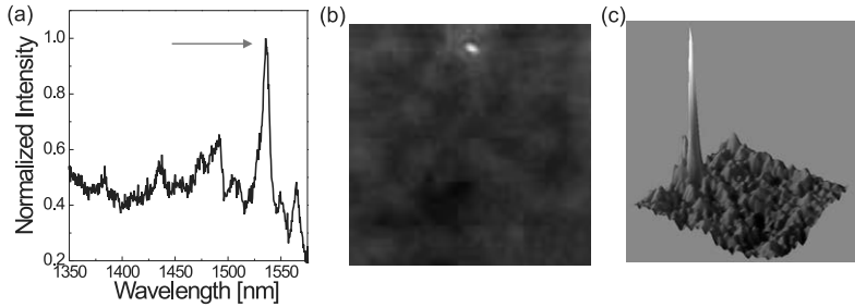
Figure 5.6: (a) Example of a near-field spectrum obtained in the Sample 1. (b) Spatial intensity distribution associated to the peak reported in the spectrum in (a). The spatial dimension of the images is 13.5 \times 13.5 \mu\text{m} . The spatially localized mode is well confined within the sample covering a large number of scatters. (c) Three-dimensional view of the image in (b).
