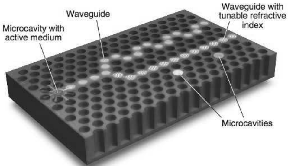
Figure 3.1: A photonic circuit can be obtained by filling the single pores of a 2D photonic crystal with liquids. Different devices can be integrated in the same sample: local light sources, bent waveguides, tunable waveguides, micro-cavities, and so on.
