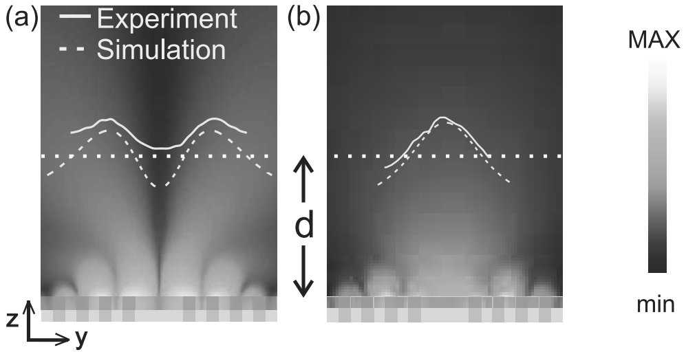
Figure 3.12: (a) and (b), Distribution of the intensity of the electric field component along the x -axis collected in a vertical plane along the y -direction and centered in the middle of the cavity (image size 2.3 \times 3 \mu\text{m} ) for the two cavity modes at 1315nm and for the broadened band at 1257nm. The white dotted line represents the effective height in with the simulated profile of the electric field (yellow dotted line) is collected. The yellow continuous lines represent the normalized experimental profile of the photonic crystal cavity mode.
