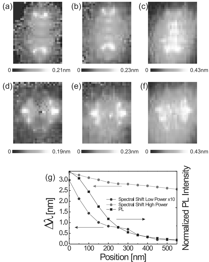
Figure 2.10: (a), (b) and (c) Maps of the tip induced spectral shift of resonance M1 for different excitation power: 0.3 \text{ MW/cm}^2 , 0.7 \text{ MW/cm}^2 and 1.4 \text{ MW/cm}^2 . (d), (e) and (f) Maps of the tip induced spectral shift of resonance M2 for different excitation power: 0.3 \text{ MW/cm}^2 , 0.7 \text{ MW/cm}^2 and 1.4 \text{ MW/cm}^2 . (g) Spectral shift spatial decay of the cavity mode for a excitation density power of 5 \text{ MW/cm}^2 (blue dots, scaled by a factor 10) and 27 \text{ MW/cm}^2 (red dots). The decay rate for the case of low excitation density power is comparable with the photoluminescence spatial decay associated to the same mode (black squares, right axis).
