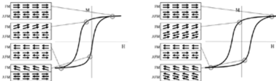
Figure 2.15: Schematic diagram of magnetic behaviour during a hysteresis loops for a AFM-FM spins system with large K_{AFM} (left) and with small K_{AFM} (right). (Nogués et al. 2005)
