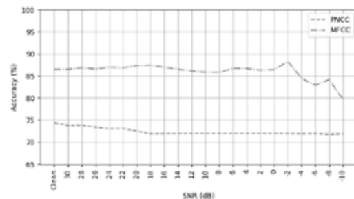
Figure 2 Classification accuracy versus SNR for polyps, actual noise random sample.
