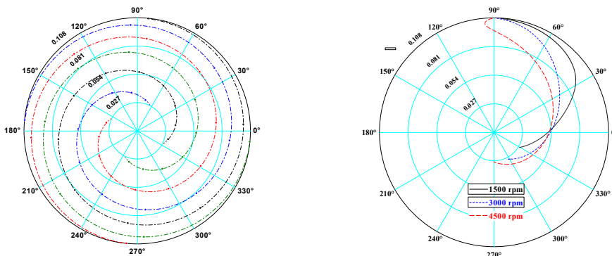
Fig. 3. 10 Absolute and relative rotor streamlines with R404a working fluid: (a) Absolute at 1500 rpm, 4 nozzles; (b) Relative streamlines at various rpm
