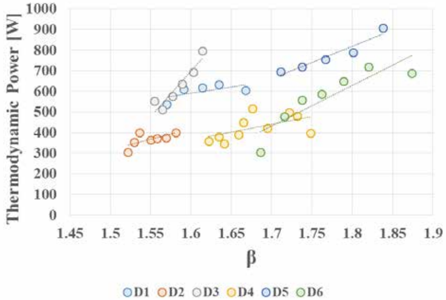
Fig. 4. 64 Experimental thermodynamic power output vs. expansion ratio
