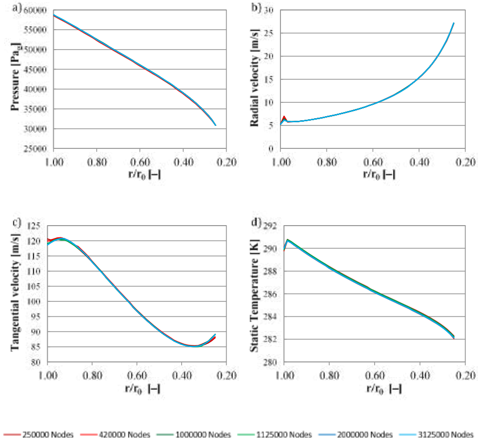
Fig. 3. 39 Results of the mesh sensitivity analysis performed on simulations with transitional turbulence model
