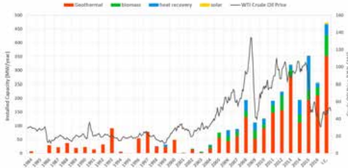
Fig. 2.8 Installed ORC capacity from 1984 up to 2017, different application highlighted (Tartière et al., 2017)
