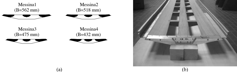
Figure 8.23 (a) Schematic drawing of the four section models and (b) picture of “Deck 1” (with spoiler)
